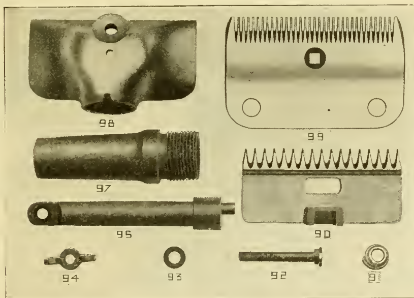
Principal Parts of Stewart Patent Clipper Knife and Handle.
