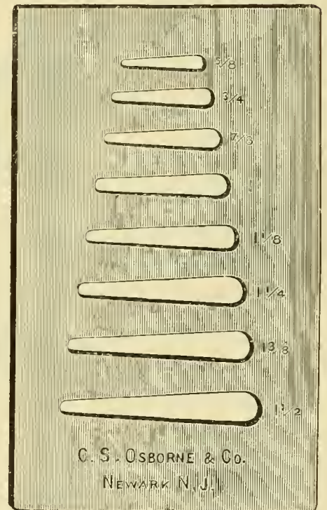
Gauges for Trace Punches.
