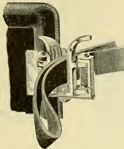
As Applied to Side of Dash.
