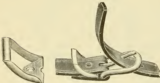
Showing Position for Upper Loops.
