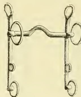
English Head Port, Four Ring with Chin Loops.
